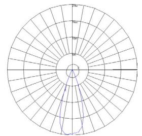
PHOTOMETRIC DIAGRAM
